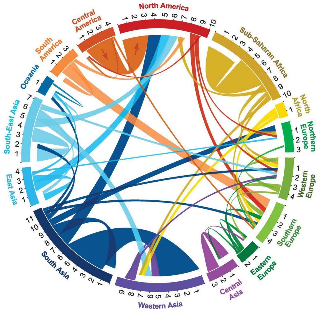
Fig. 1 Circular plot of migration flows between and within world regions during 2005 to 2010. Tick marks show the number of migrants (inflows and outflows) in millions.
